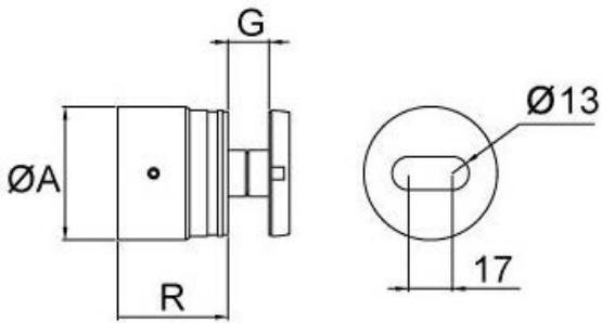
PINTERIOR HANDRAIL, HANDRAIL AND BUTTONS DETAIL
