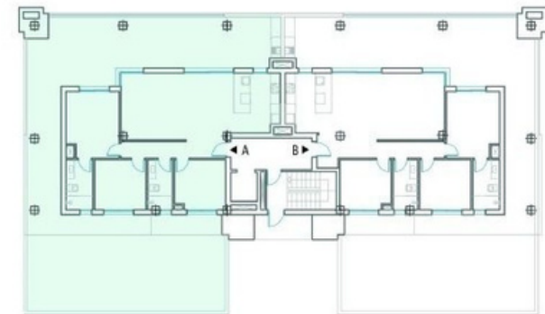
APARTMENT SURFACES APARTMENT TYPE 1A
