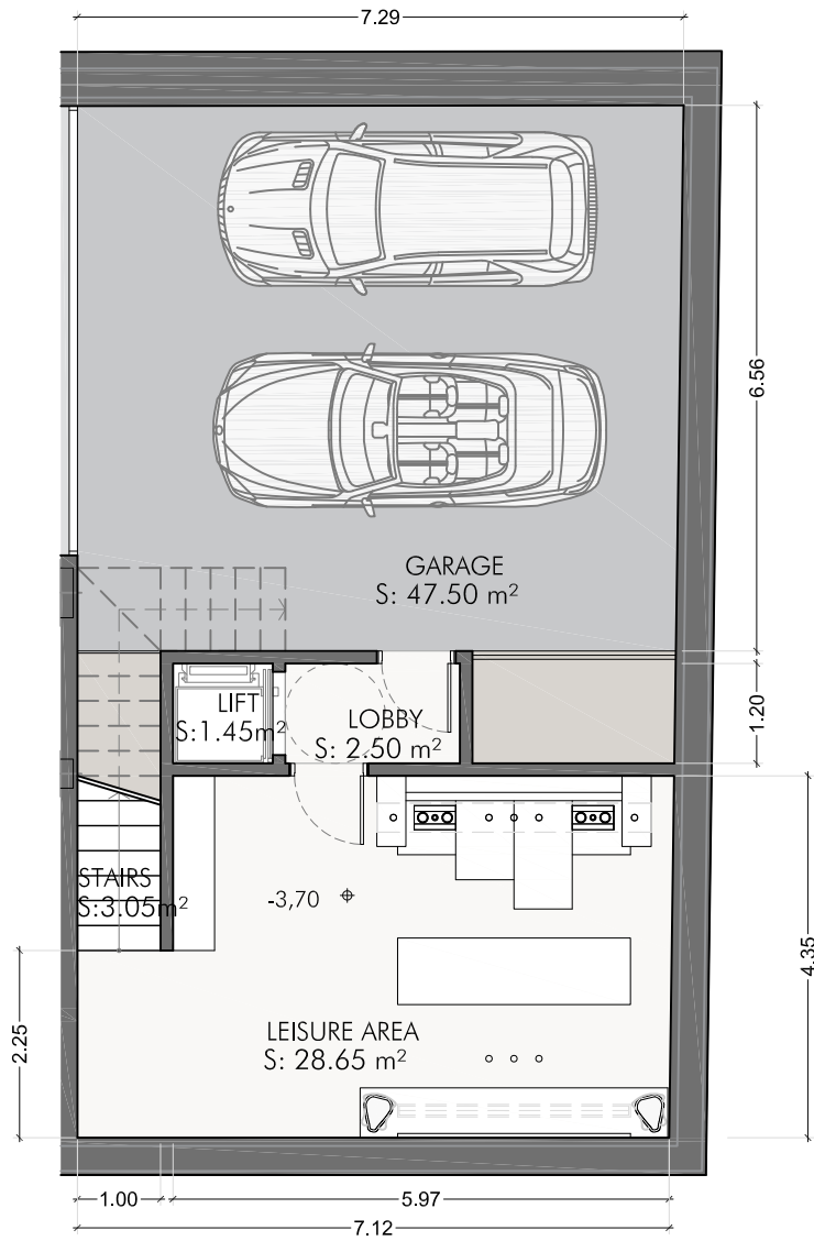
Basement
