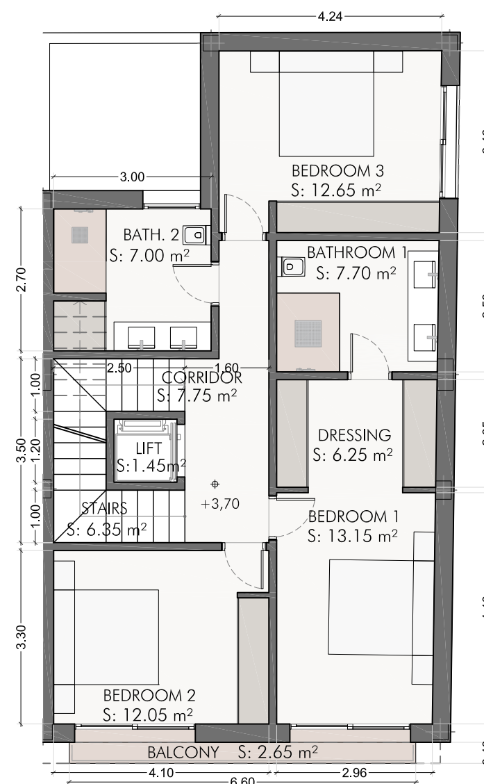
First Floor
