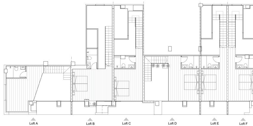
Upper Floor
