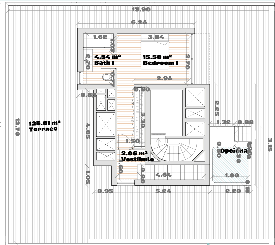
Penthouse floor Planta atico
