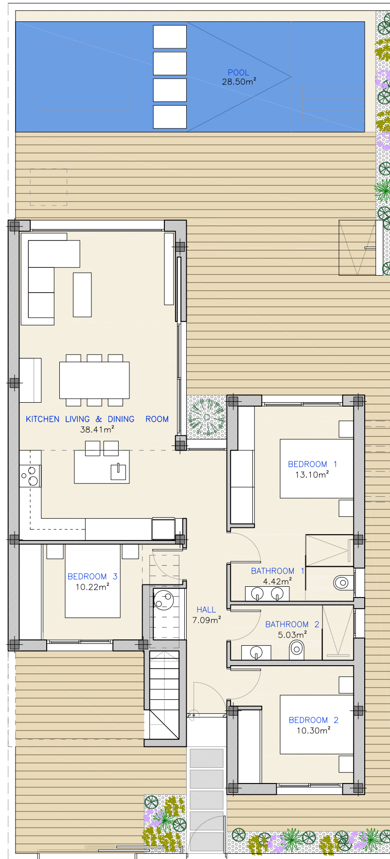
GROUND FLOOR
