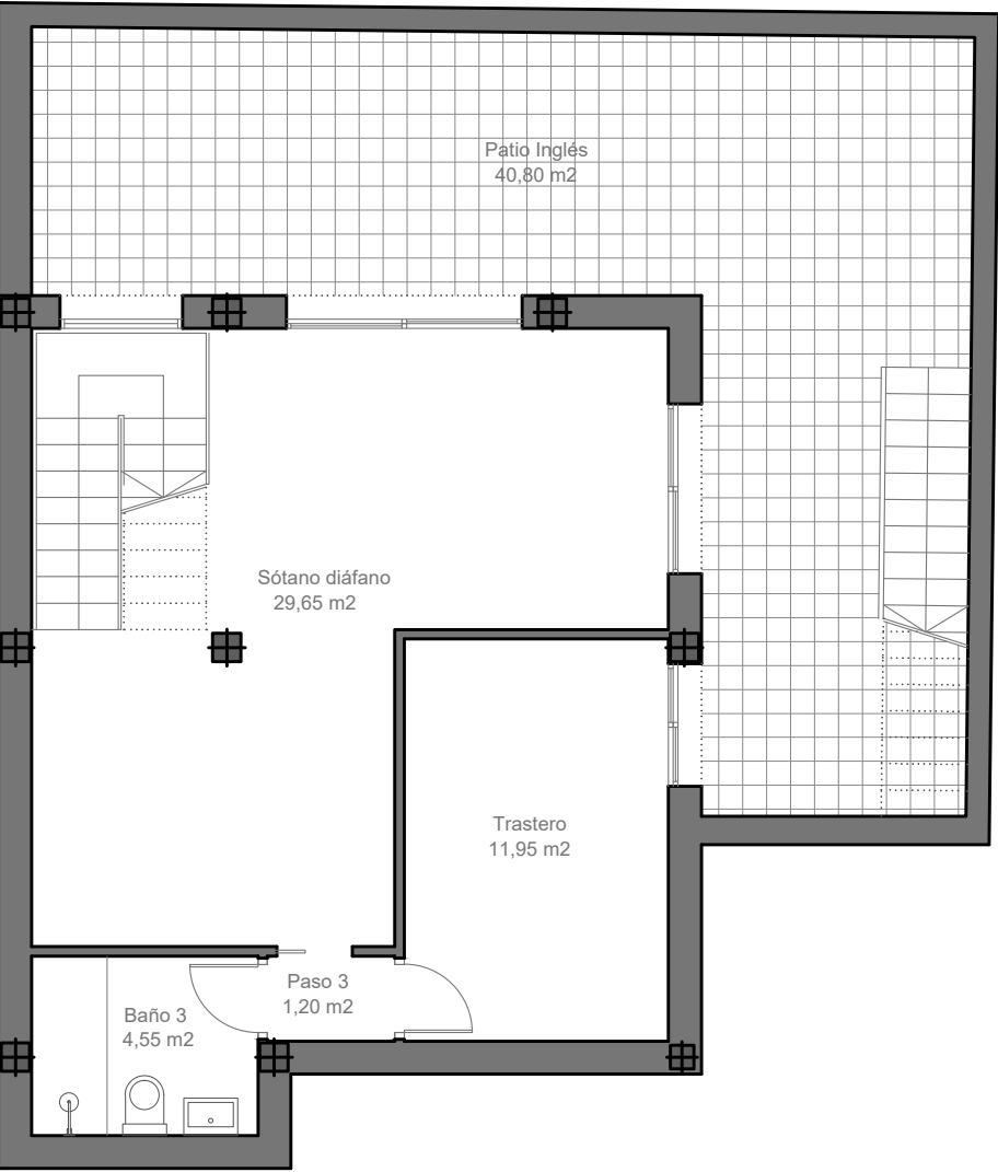
Basement floor
