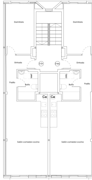
Second and Third Floor
